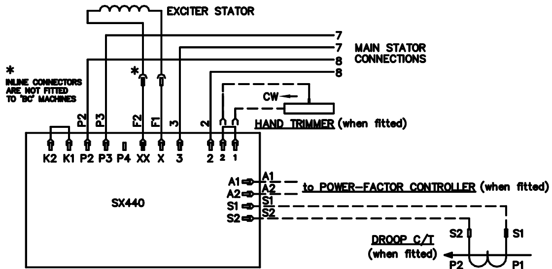
Fig 1 : Existing AVR wiring.
